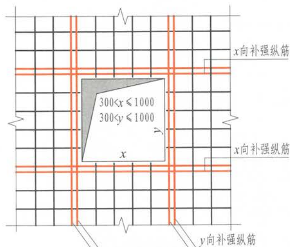
(a) 板中开洞
