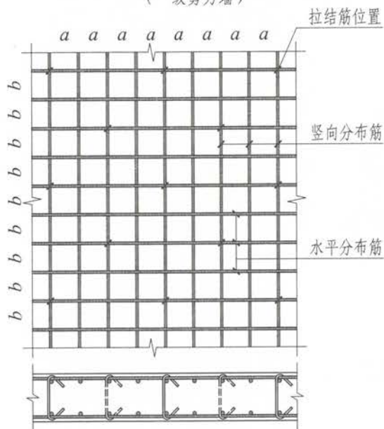
(a) 拉结筋@4a@4b梅花 (a ≤ 150, b ≤ 150)
