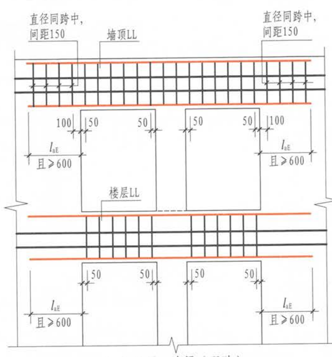
(c) 双洞口连梁 (双跨)
