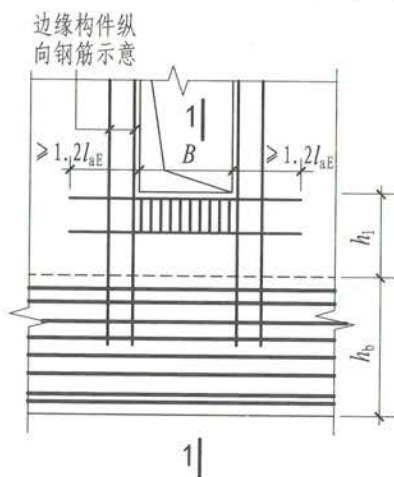
(B ≤ 2h 1 且 h 1 ≥ h b /2)
