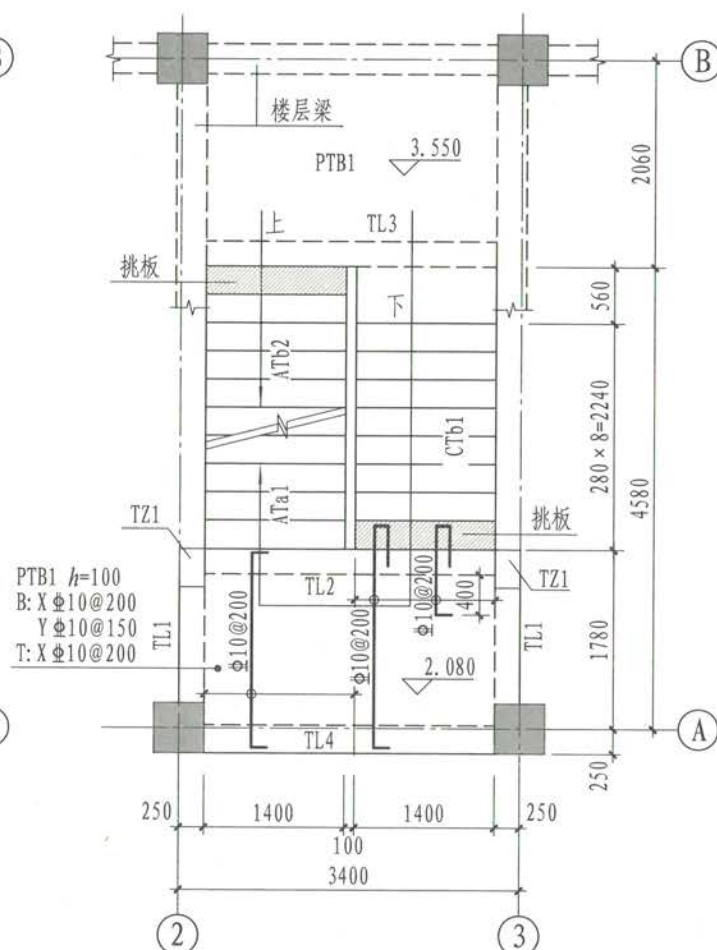
▽2.080~▽3.550楼梯平面图
