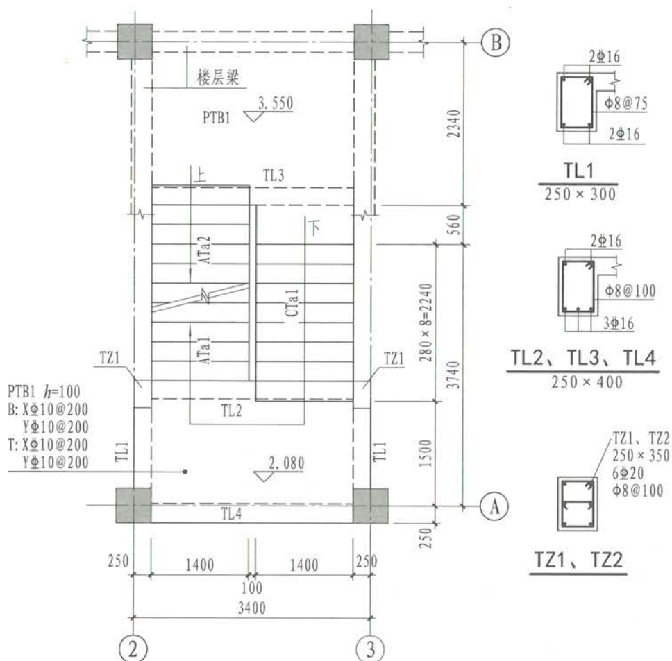
▽2.080~▽3.550楼梯平面图
