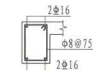
TL1 250 × 300
